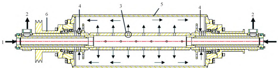
1-cooling water inlet; 2-cooling water outlet; 3-water outlet hole; 4-reflow hole; 5-water-cooled roller; 6-pulley
