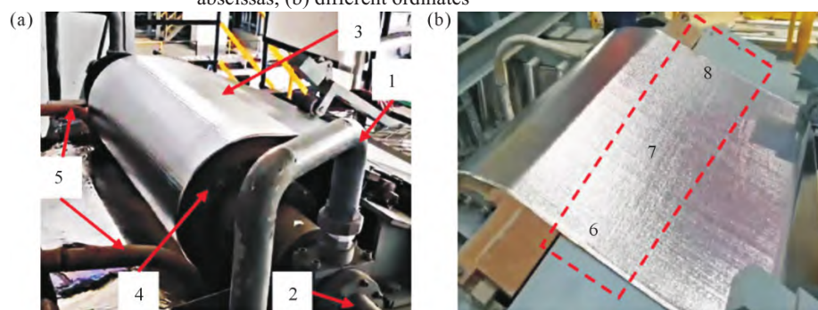
1-water inlet pipe; 2-outlet pipe; 3-lead sheet; 4-water-cooled rollers; 5-lead pump
