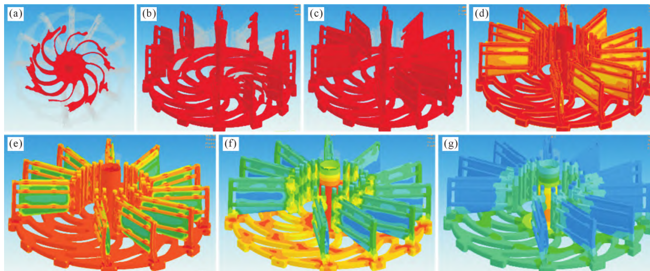
图 3 金属液流动路线和充型过程温度场变化:(a) 0.7 s; (b) 3.4 s; (c) 5.6 s; (d) 15.1 s; (e) 30.0 s; (f) 110.1 s; (g) 530.1 s Fig.3 Variation in the temperature field during metal liquid flow and mold filling process in casting: (a) 0.7 s; (b) 3.4 s; (c) 5.6 s; (d) 15.1 s; (e) 30.0 s; (f) 110.1 s; (g) 530.1 s
