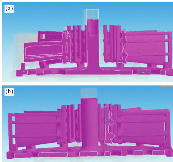
图 6 缺陷模拟结果:(a)凝固中;(b)凝固结束 Fig.6 Simulation results of defects: (a) during solidification; (b) solidification completed
