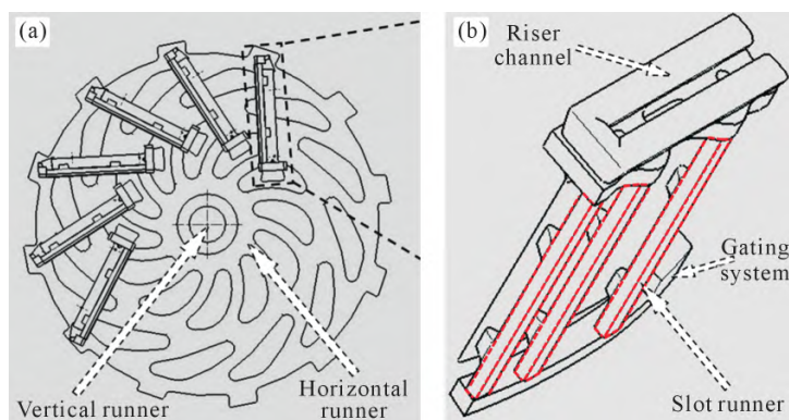
图 2 浇注系统示意图:(a) 平面结构;(b) 支板放大图 Fig.2 Schematic diagram of the pouring system: (a) planar structure; (b) enlarged view of the support plate
