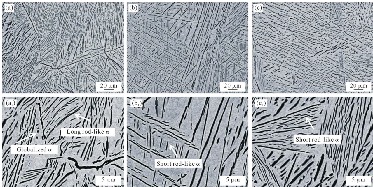
图 8 Ti-62222 钛合金在变形温度为 930 °C、变形量为 60%变形后的微观组织:(a, a 1 ) 0.1 s -1 ; (b, b 1 ) 0.01 s -1 ; (c, c 1 ) 0.001 s -1 Fig.8 Microstructure of Ti-62222 at a deformation temperature of 930 °C and a deformation of 30%:(a, a 1 ) 0.1 s -1 ; (b, b 1 ) 0.01 s -1 ; (c, c 1 ) 0.001 s -1
