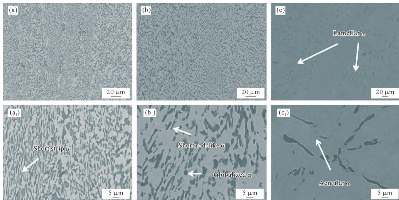
图3 Ti-62222 合金在变形量为 60%、应变速率为 0.001 \text{ s}^{-1} 变形后的微观组织:(a, a 1 ) 860 °C; (b, b 1 ) 890 °C; (c, c 1 ) 930 °C Fig.3 Microstructure of Ti-62222 with a strain rate of 0.001 \text{ s}^{-1} and a deformation of 60% at different temperatures: (a, a 1 ) 860 °C; (b, b 1 ) 890 °C; (c, c 1 ) 930 °C
