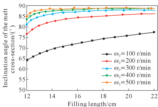
图4 倾角随充型长度的变化 [10] Fig.4 Variation in inclination angle with filling length [10]
