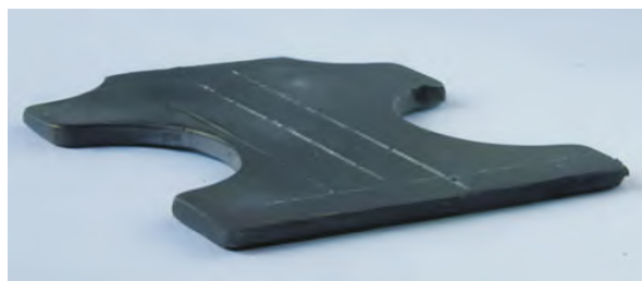
图5 Ti-43Al-9V 填充 1.3 mm 薄壁件 [7] Fig.5 Thin-walled parts (1.3 mm thick) filled with Ti-43Al-9V [7]
