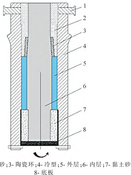
图 16 辊身冷型及辊颈造型整体示意图 [58] Fig.16 Overall schematic diagram of roll body cooling and roll neck modelling [58]
