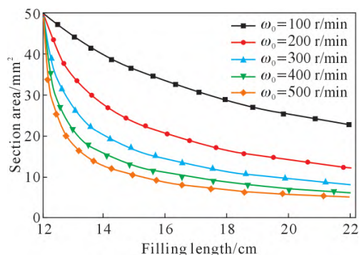
图3 截面面积随充型长度的变化 [10] Fig.3 Variation in section area with filling length [10]
