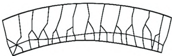
图2 离心铸管环形中心缩松带 [6] Fig.2 Shrinkage band in the center of the centrifugally cast pipe ring [6]
