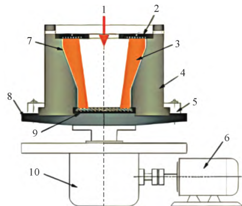
图 18 变径管立式离心浇注装置示意图 [62] Fig.18 Schematic diagram of the vertical centrifugal casting device for reducing pipes [62]
