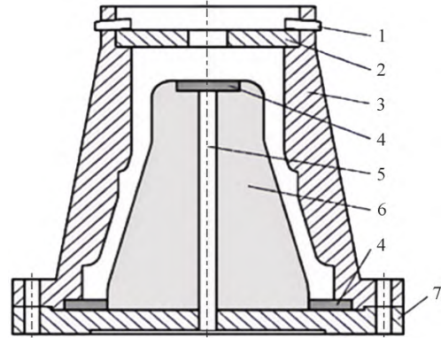
图 17 改进型立式离心铸造用铸型结构示意图 [61] Fig.17 Schematic diagram of the improved vertical centrifugal casting model structure [61]
