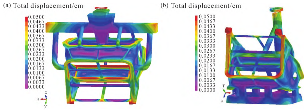
图 7 不同浇注方式下位移分布:(a) 顶注式;(b) 底注式 Fig.7 Displacement of castings processed with different gating systems: (a) top gating system; (b) bottom gating system
