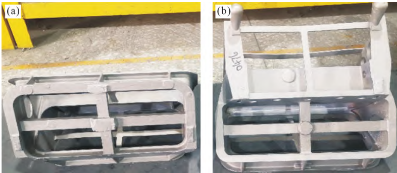
图 8 铸件毛坯:(a) 顶注式;(b) 底注式 Fig.8 Castings processed with different gating systems: (a) top gating system; (b) bottom gating system
