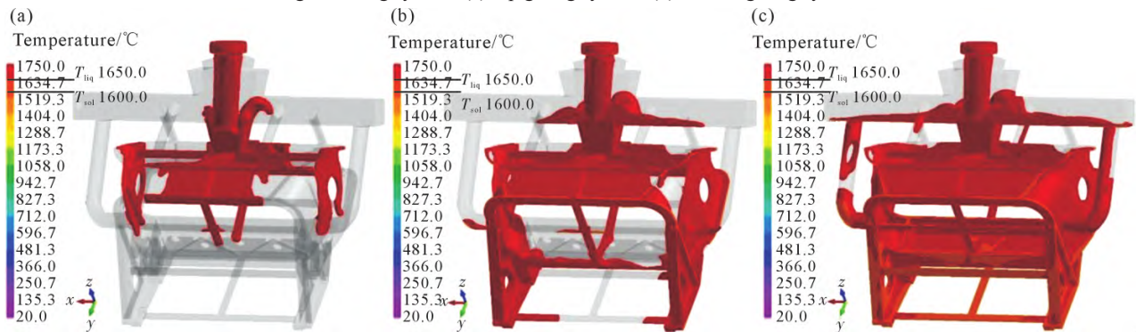
图3 顶注充型过程:(a) t=0.6 s; (b) t=1.02 s; (c) t=1.78 s
