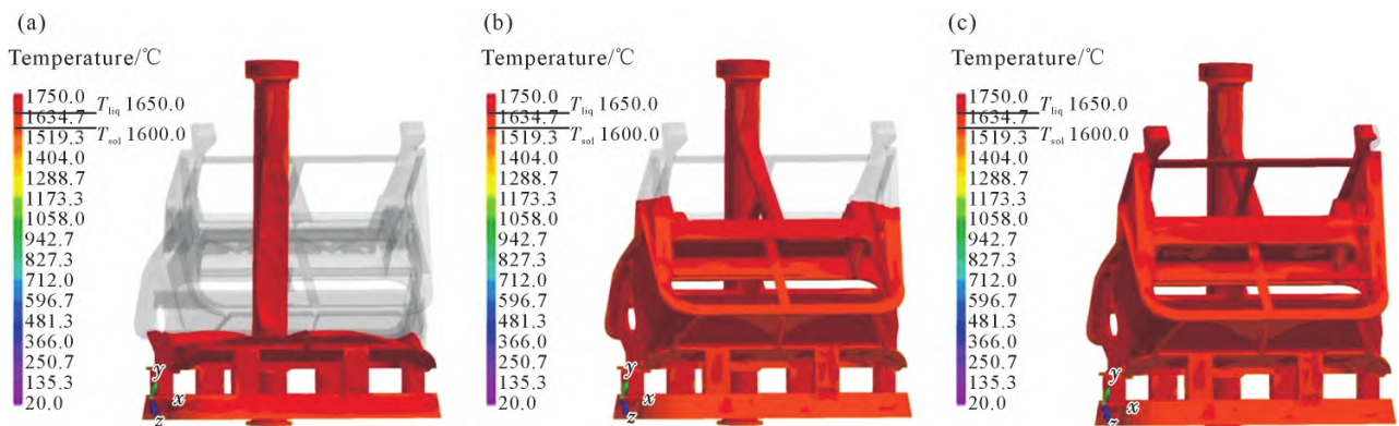
图4 底注充型过程:(a) t=1.68 s; (b) t=2.17 s; (c) t=2.81 s
