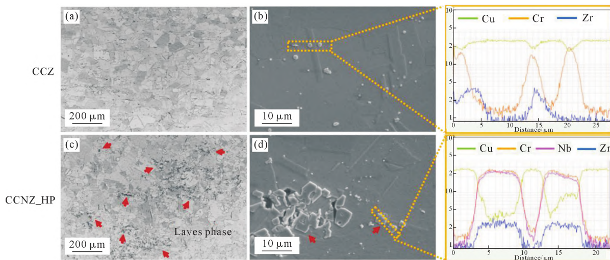
图 8 时效条件下 Cu-Cr-Zr 和 Cu-Cr-Nb-Zr 合金:(a,c) 晶粒形貌的光学显微组织,(b,d) 带有线扫描结果的 SEM 图像 [62] Fig.8 Cu-Cr-Zr and Cu-Cr-Nb-Zr alloys under as-aged conditions: (a,c) optical microstructures showing the grain morphologies, (b,d) SEM images with inset line scan results [62]
