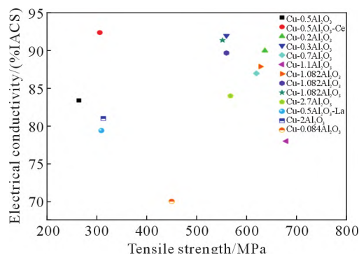
图 11 部分 Cu-Al 2 O 3 合金的抗拉强度和导电性能 [84-85,87-92] Fig.11 Tensile property and electrical conductivity diagram of several Cu-Al 2 O 3 alloys [84-85,87-92]
