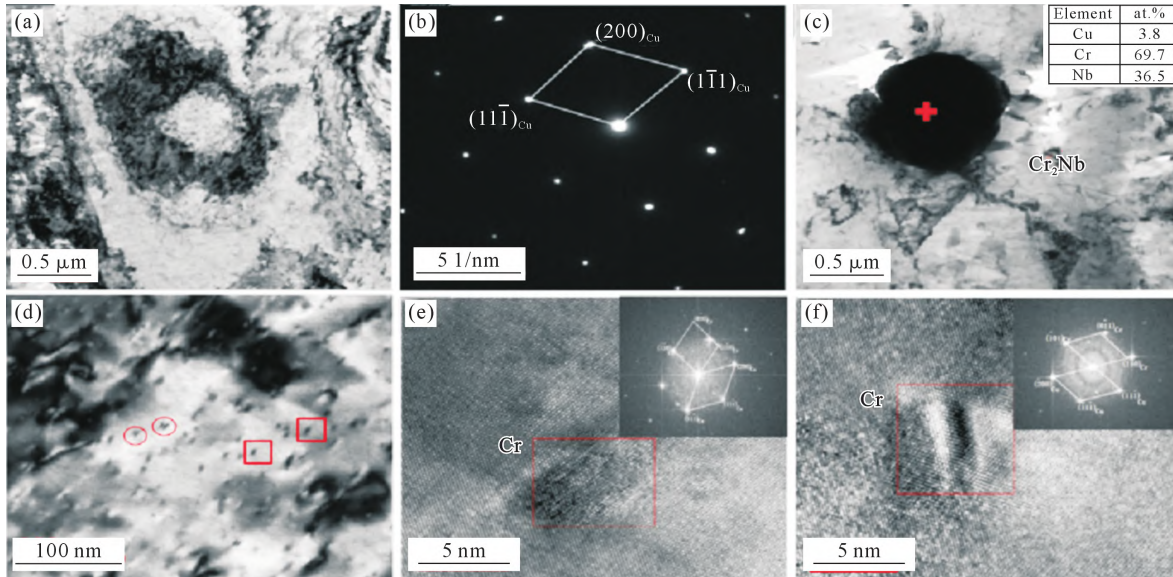
图9 450 °C时效4 h的Cu-Cr-Nb合金:(a~d) TEM明场像,(b)选区电子衍射图谱,(e~f) HRTEM图像 [71] Fig.9 Cu-Cr-Nb alloy aged at 450 °C for 4 h: (a~d) TEM bright-field images, (b) SAED pattern, (e~f) HRTEM images [71]
