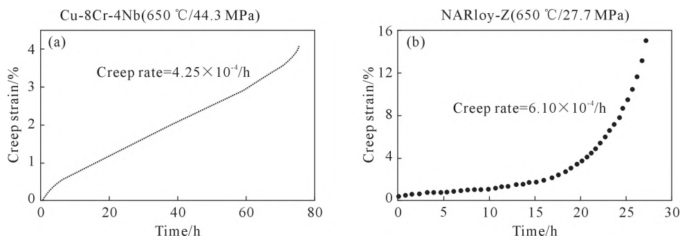
图10 合金典型蠕变曲线:(a) Cu-8Cr-4Nb, (b) NARloy-Z [73] Fig.10 Typical creep curves of alloys: (a) Cu-Cr-Nb, (b) NARloy-Z [73]
