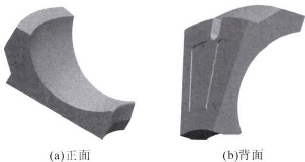
图 1 衬板铸件形状示意图 Fig.1 Schematic diagram of typical liner casting structure
