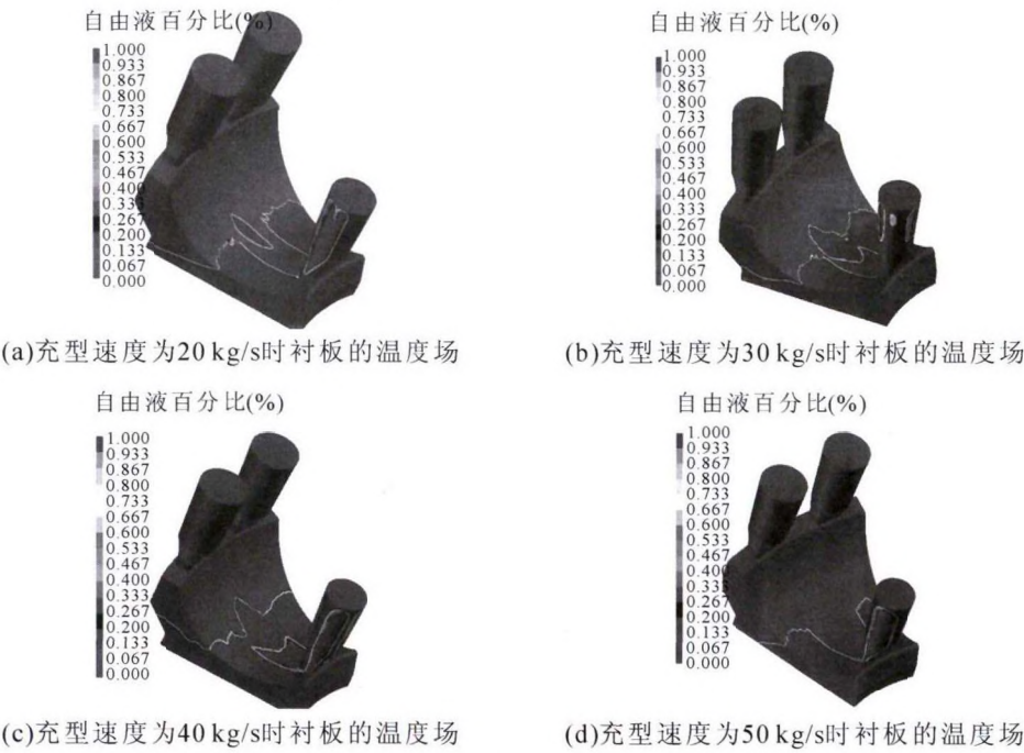
图 4 不同充型速度下衬板的温度场 Fig.4 Typical lining casting temperature field under different filling speed
