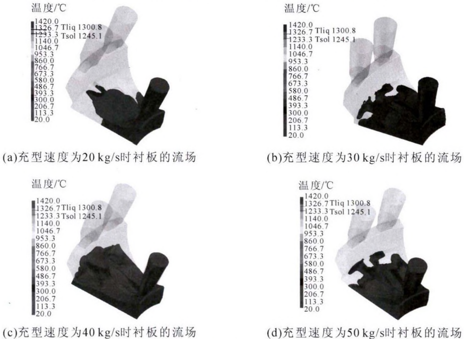
图 5 不同充型速度下衬板的流场 Fig.5 Typical lining casting flow field under different filling speed
