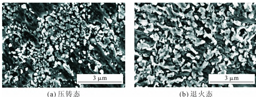
图3 压铸态和退火态 AlSi7MgMn 合金共晶区域的微观组织 SEM 形貌 Fig.3 SEM image of microstructure of eutectic region in as die cast and annealed AlSi7MgMn alloy
