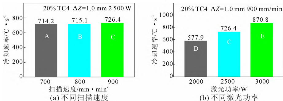
图 4 不同扫描速度和激光功率下的凝固冷却速率 Fig.4 Solidification cooling rate under different scanning speed and laser power
