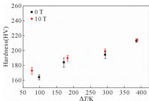
图5 有无磁场下 CrCoNi 合金不同过冷度凝固时的硬度图 Fig.5 The hardness of CrCoNi alloy solidified at different undercoolings with and without magnetic field
